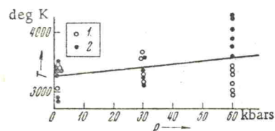
Fig. 1. Melting curve of tantalum: 1) I_1/I_2 ; 2) I_2/I_3 .
